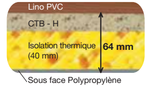
Plancher "ISOTHERM 64"
